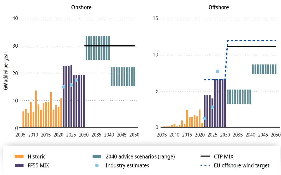
Figure 17 Indicators E4b and E4c – annual wind electricity capacity additions
